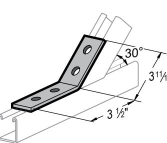
4-HOLE 30° CORNER ANGLE L45
