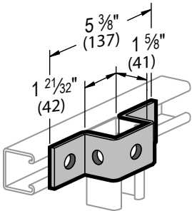
5 HOLE U SUPPORT U10
