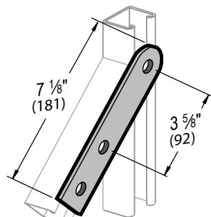
3 HOLE SWIVEL PLATE F27
