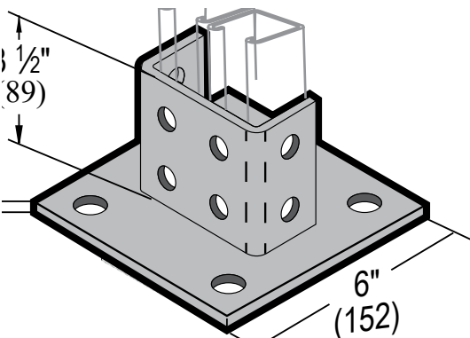
POST BASE SQUARE FOR A12A SP13SQ
