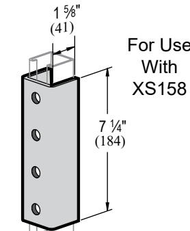
4 HOLE SPLICE CLEVIS U24
