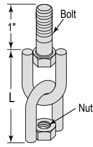
FEMALE-MALE SWIVEL SWMF
