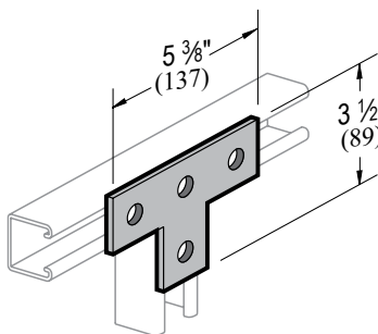
4 HOLE TEE PLATE F25
