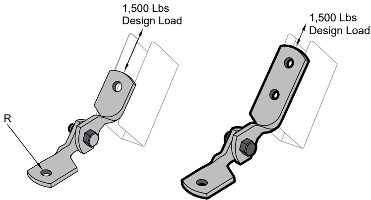
4 HOLE SPLICE PLATE H502
