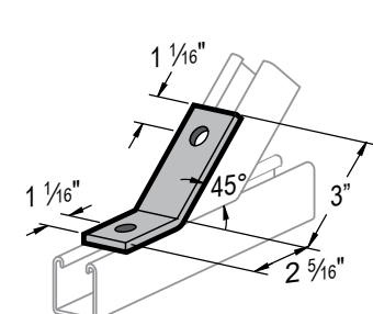
2-HOLE 45° CORNER ANGLE L46
