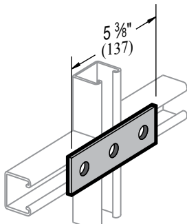
3 HOLE SPLICE PLATE F20
