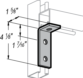
3 HOLE 1-5/8" X 4-1/8" CORNER ANGLE L20
