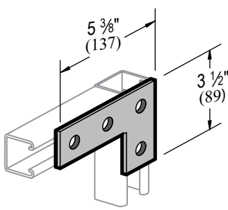
3 HOLE SWIVEL PLATE F37
