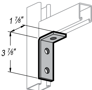
3 HOLE 1-7/8" X 3-7/8" CORNER ANGLE L19
