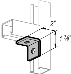
2-HOLE 2" X 1-7/8" 90° CORNER L11
