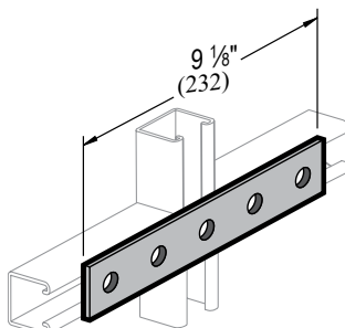
5 HOLE SPLICE PLATE F21
