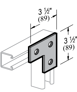
2 HOLE SWIVEL PLATE F36
