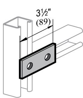
2 HOLE SPLICE PLATE F09
