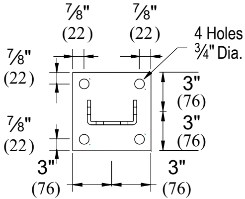
POST BASE FLUSH FOR A12A SP13FL
