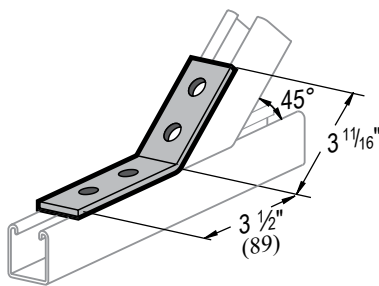
4-HOLE 45° CORNER ANGLE L220045
