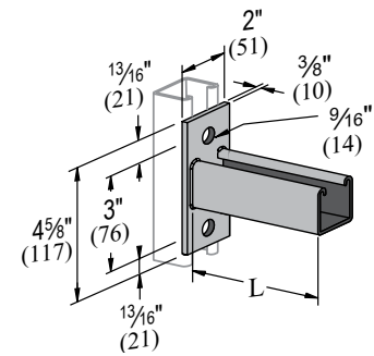
SGL STRUT BRACKET BR22
