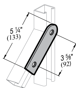
2 HOLE SWIVEL PLATE F26
